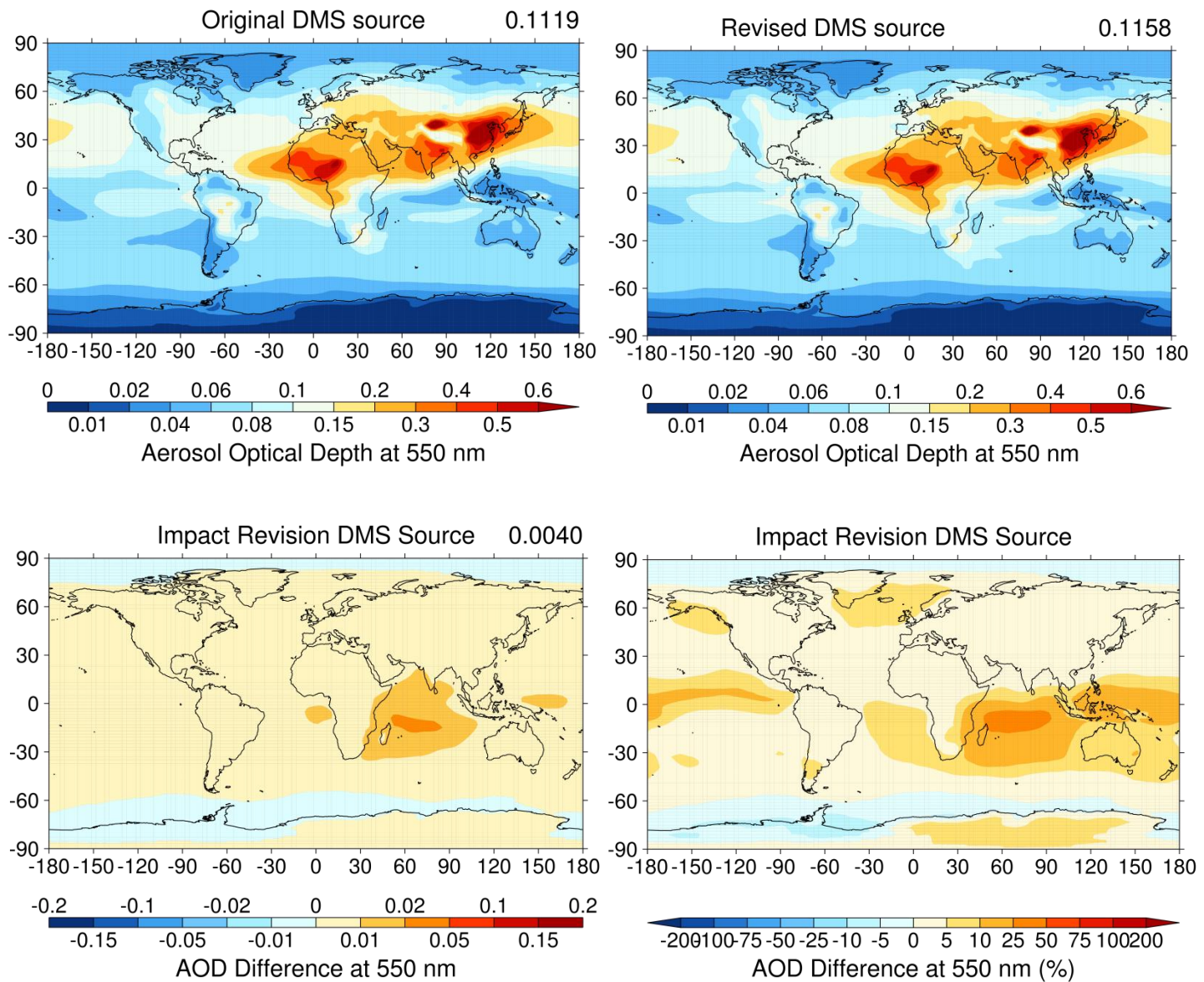
Figure 3. Aerosol optical depths obtained with the old and new description of the DMS source (top panels), together with the absolute and relative differences (new minus old).
