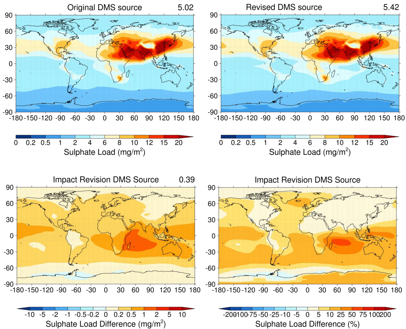
Figure 3. Sulphate loads obtained with the old and new description of the DMS source (top panels), together with the absolute and relative differences (new minus old).
