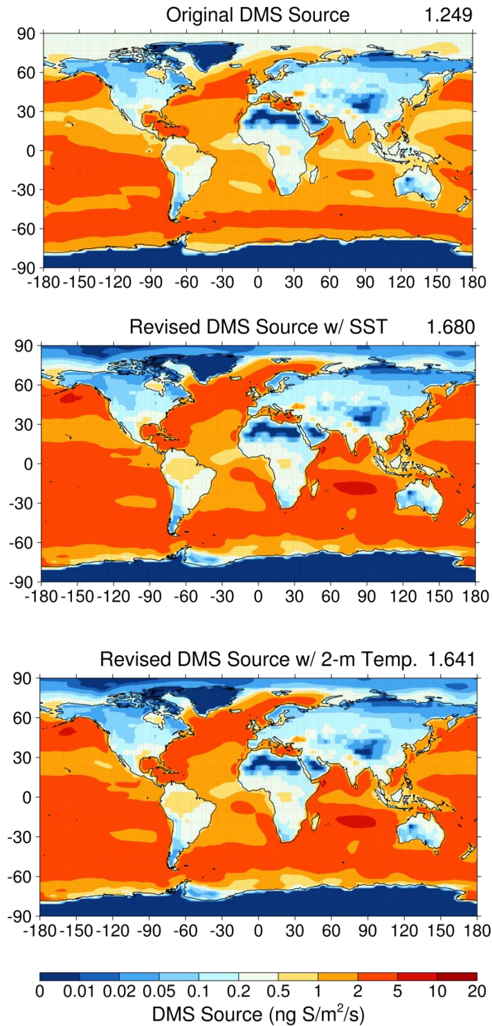
Figure 1. Annual mean DMS flux for the old implementation (top panel), the new implementation using the actual sea surface temperatures (middle panel), and the new implementation with SSTs approximated by 2 m air temperatures (bottom panel).
